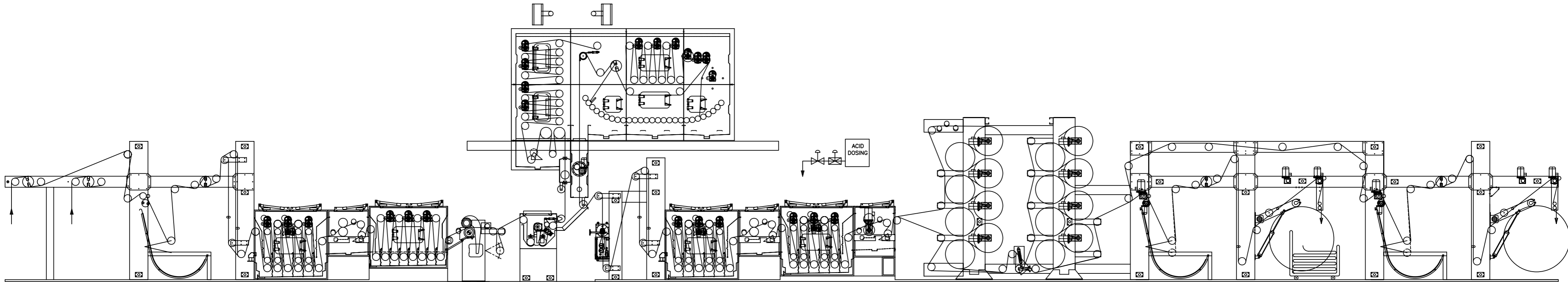
FEEDING S.S.SCRAY WITH FEEDING "S" CLOSE TANK MANGLE NORMAL CLOSE TANK 10 TON NIP APPLICATOR SCROLL ROLL #150 "S" CLOSE TANK MANGLE CLOSE TANK WELDED PARTITION MANGLE 18+2 CYLINDER DRYING RANGE S.S.SCRAY PLAITER WITH BIGBATCHING S.S.SCRAY PLAITER WITH BIGBATCHING
