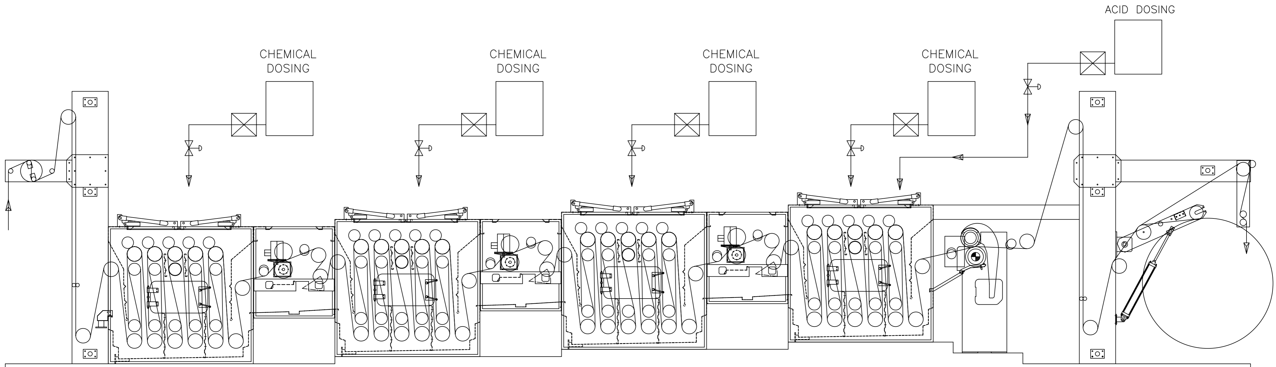
FEEDING "S"TYPE CLOSE TANK MANGLE (ø250) "S"TYPE CLOSE TANK MANGLE "S"TYPE CLOSE TANK MANGLE "S"TYPE CLOSE TANK 10TON NIP PLAITER WITH BIG BATCHING
